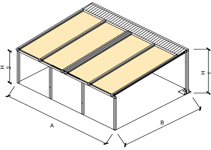
PERGOLA PERSPECTIVE
