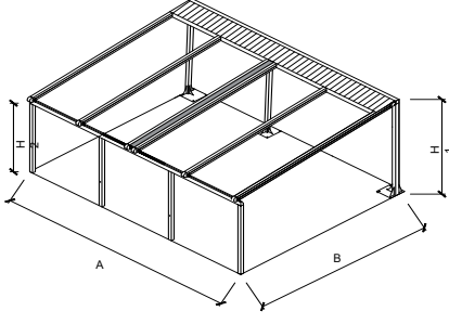
PERGOLA CONSTRUCTION PERSPECTIVE
