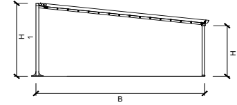
PERGOLA SIDE VIEW
